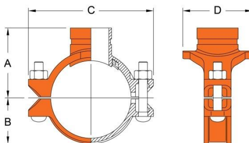
Model M22 Mechanical Tee, Grooved-End Outlet
